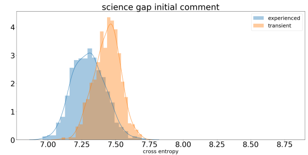
Figure 4. Sampled distribution of cross entropies between first time comments of users who leave and who stay. Difference is significant ( p < .001 ).
