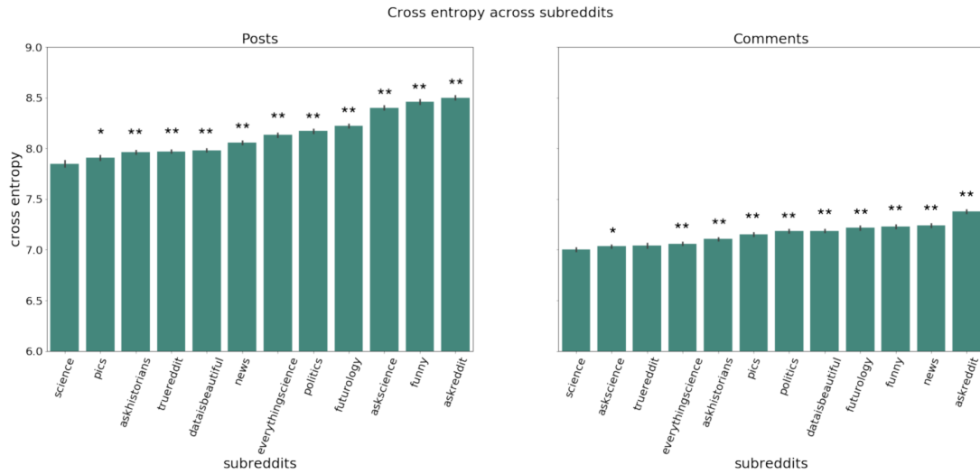
Figure 2. Cross entropies of posts and comments from experienced contributors from each subreddit, calculated using r/science language models. Bars show bootstrapped 95% confidence intervals. Asterisks denote t -test significance compared to r/science . Similar results were found using Mann-Whitney U tests for non-normal distributions. All results are corrected for multiple hypothesis testing using Bonferroni-Holm; * p < .05, ** p < .001.
