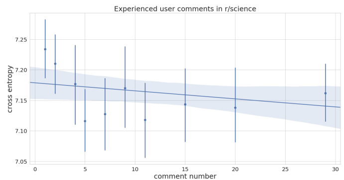
Figure 6. Cross entropy of contributors as they contribute more to r/science . Cross entropies are binned into 10 equal groups of comments. Correlation is significant using Spearman's rank-order correlation ( \rho = -0.027 , p < .01 ).
